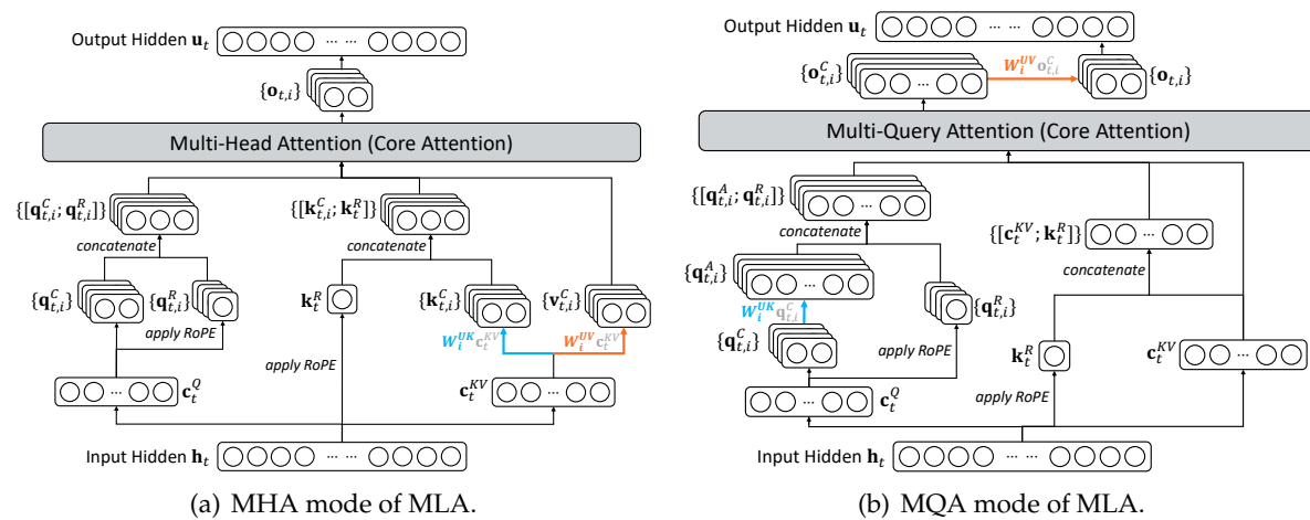
Figure 7 | Illustration of the MHA and MQA modes of MLA. For DeepSeek-V3.1-Terminus, the MHA mode is used for training and prefilling, while the MQA mode is used for decoding.
